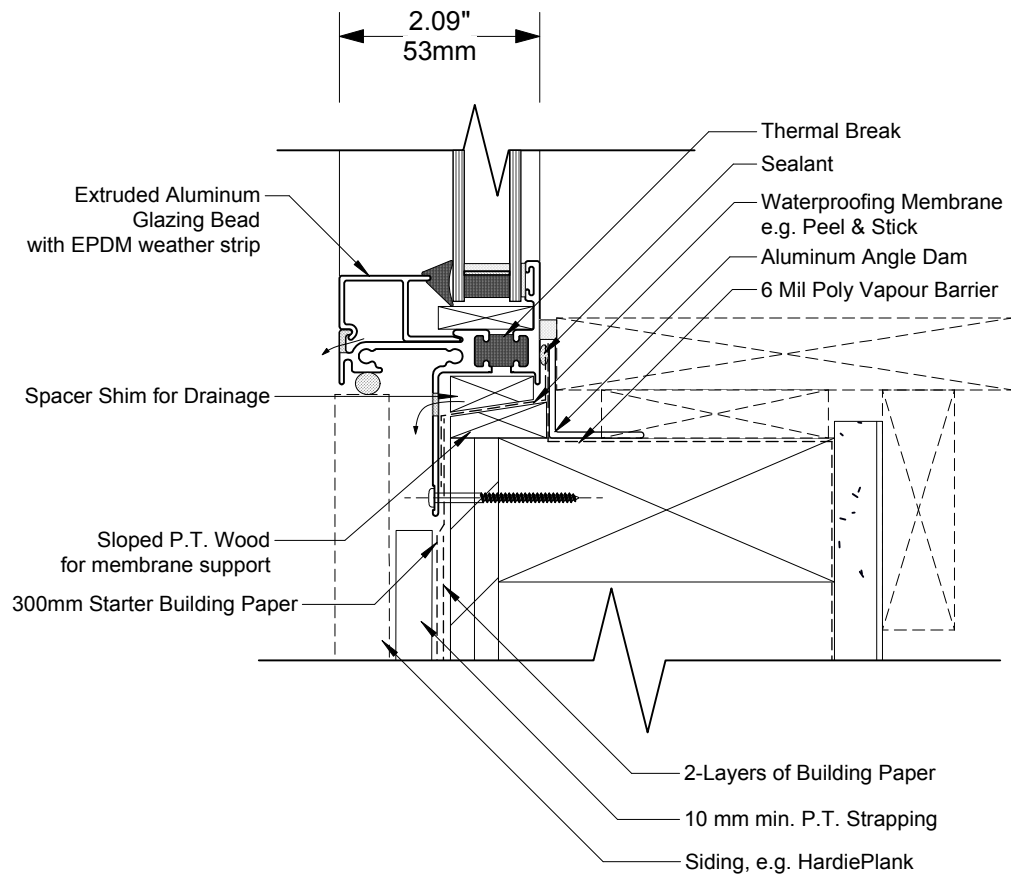
3 Picture Sill Detail Scale: 1:2
